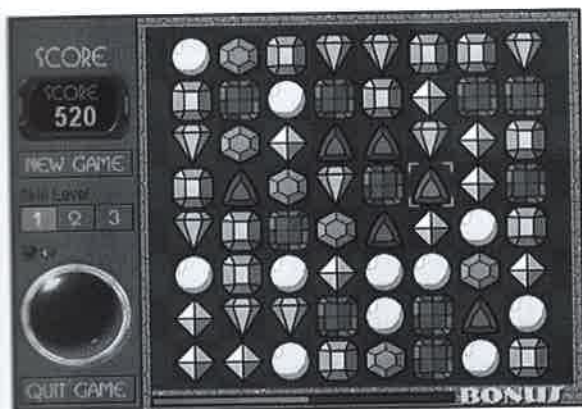
3.14 Alignment: Bejeweled
